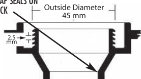
Thread Cutaway
