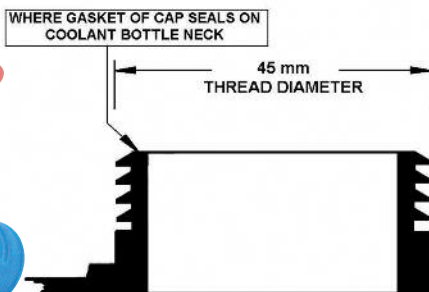
COOLING SYSTEM TANK THREAD CUTAWAY
