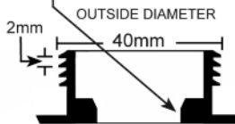
Thread Cutaway
