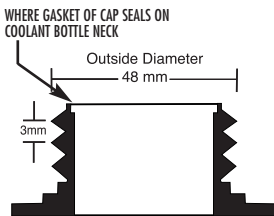
Thread Cutaway
