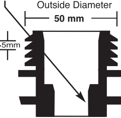
Thread Cutaway
