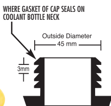
Thread Cutaway
