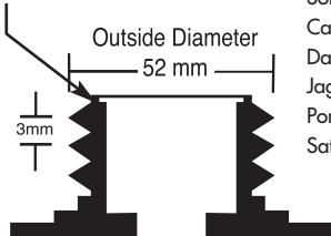
Thread Cutaway
