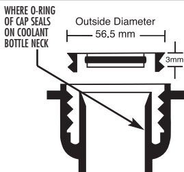
Thread Cutaway
