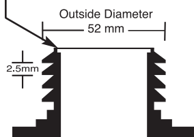
Thread Cutaway
