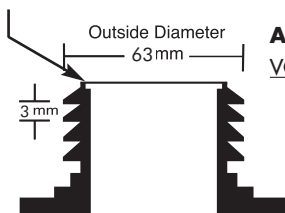
Thread Cutaway
