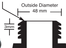
Thread Cutaway
