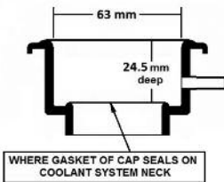
Thread Cutaway
